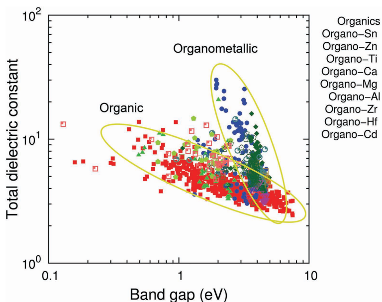
Figure 16. Computed dielectric constant of more than one thousand organic and organometallic materials, shown again their computed bandgap. Two ovals are used to indicate the different regions occupied by the organic and organometallic materials. The data used in this figure were taken from ref. [63].
