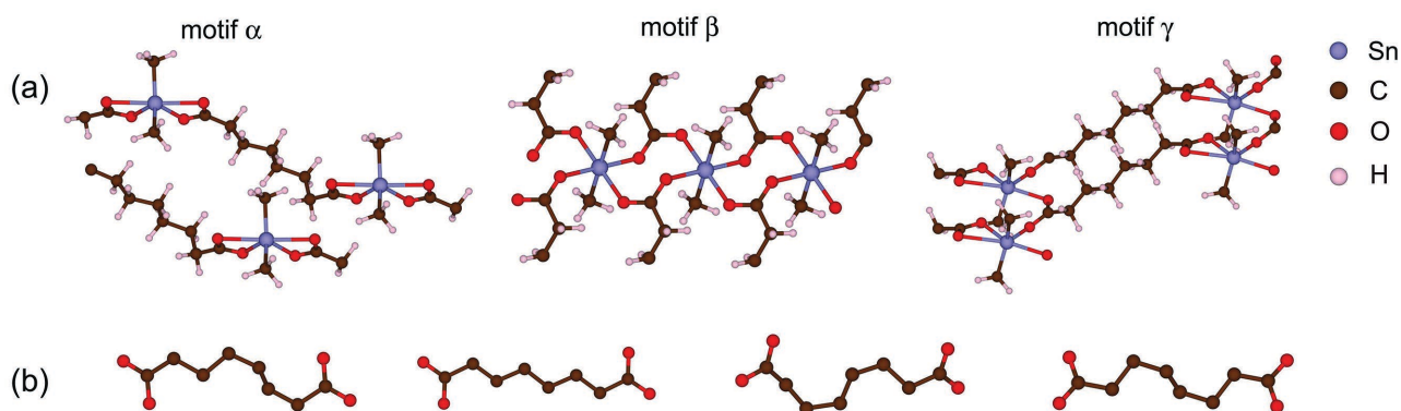
Figure 13. a) Three basic structural motifs ( \alpha , \beta , and \gamma ) computationally predicted for poly(dimethyltin esters). b) Some folding patterns of the methylene linker. Reproduced with permission. [17] Copyright 2015, American Chemical Society.
