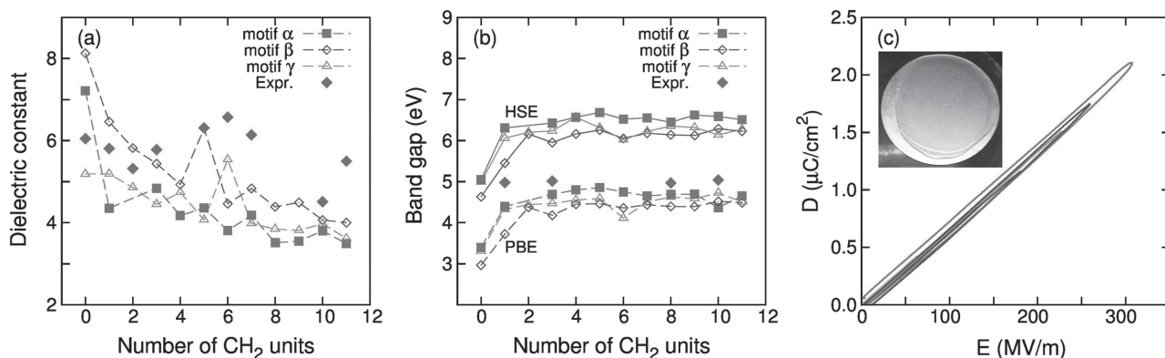
Figure 14. Computed and measured data for: a) dielectric constants and b) bandgaps (calculated at PBE and HSE levels of theory) of the poly(dimethyltin esters) in different motifs ( \alpha , \beta , and \gamma ) with different linker lengths, ranging from 0 to 11 methylene ( \text{CH}_2 ) units. In (c), the D–E loops measured for the 20/80 (wt/wt) blend of pDMTSub/pDMTDMG are shown together with a film cast for this polymer in the inset. Figure 14 is plotted from the data reported in ref. [17].
